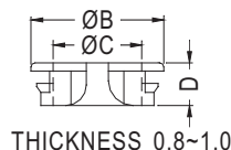
MOUNTING HOLE
