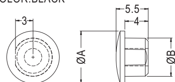
ONLY FOR : MHD-10I MOUNTING HOLE: ØC
