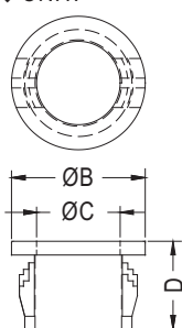
MOUNTING HOLE
