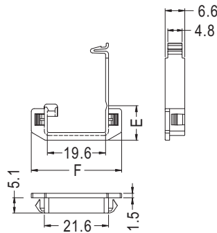
THROUGH HOLE INSTALLATION EDGE INSTALLATION
