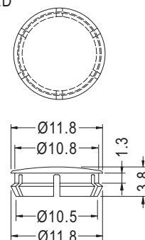
MOUNTING HOLE Ø11
