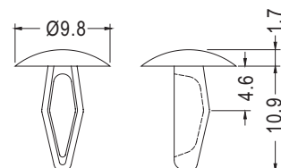
CHASSIS Ø3.9~Ø4.05 THICKNESS 2.1~3.7
