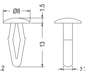
CHASSIS Ø3.9 THICKNESS 1.0~5.0
