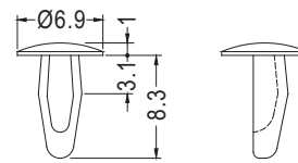
CHASSIS Ø3.1~Ø3.2 THICKNESS 2.0~2.5
