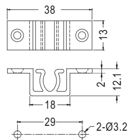
MOUNTING HOLE
