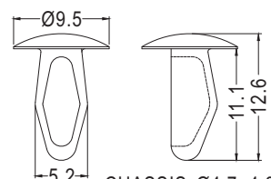
CHASSIS Ø4.7~4.8 THICKNESS 2.5~4.0
