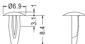
CHASSIS Ø3.1~Ø3.2 THICKNESS 2.0~2.5
