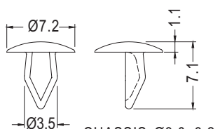
CHASSIS Ø3.0~3.2 THICKNESS 0.8~2.0
