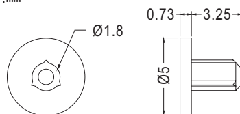
CHASSIS Ø1.8~Ø2.0
