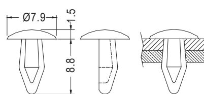
CHASSIS Ø3.5~Ø3.7 THICKNESS 3.5~4.0
