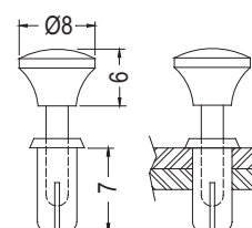
CHASSIS Ø4.1 THICKNESS 4.5~5.5
