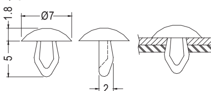
CHASSIS Ø3.15~Ø3.2 THICKNESS 1.6~1.9
