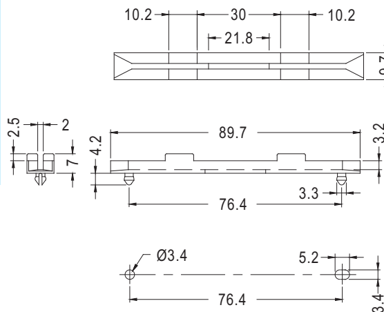
MOUNTING HOLES
