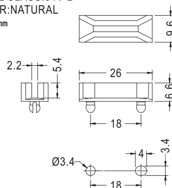
MOUNTING HOLES
