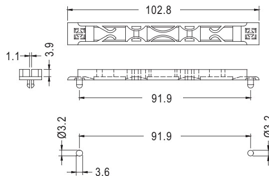
MOUNTING HOLES CHASSIS THICKNESS 1.6~2.2
