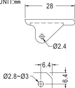
MOUNTING HOLE
