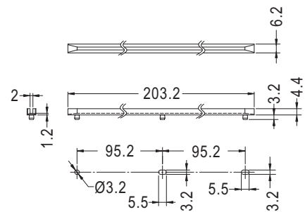
MOUNTING HOLES CHASSIS THICKNESS 1.2~2.0mm
