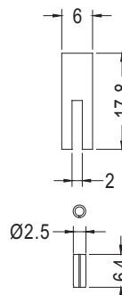
PIN
